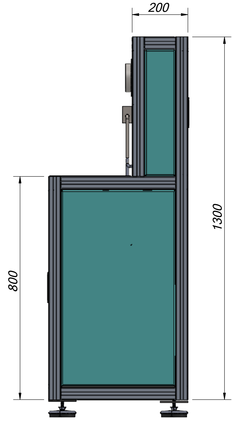
SIDE VIEW
