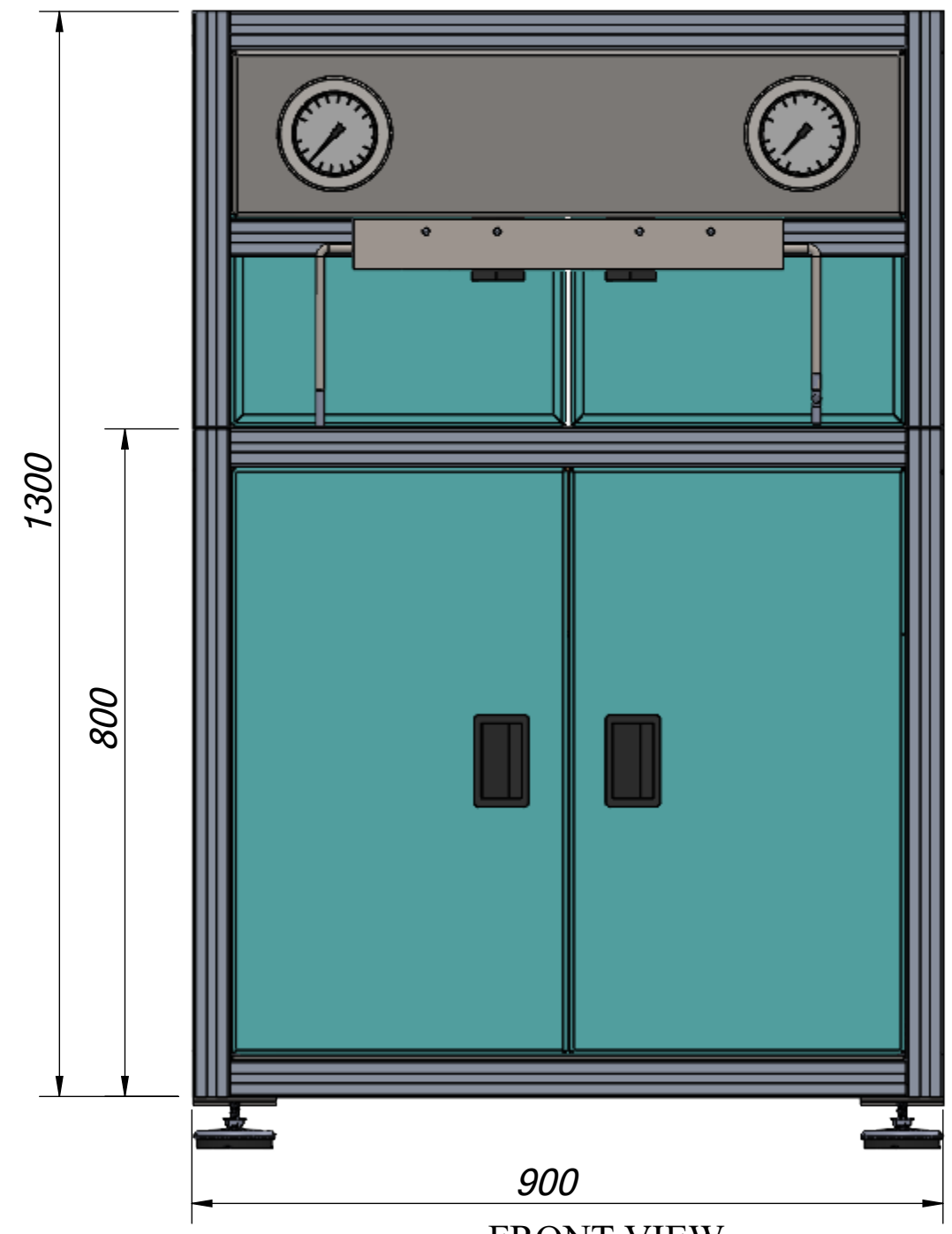
FRONT VIEW
