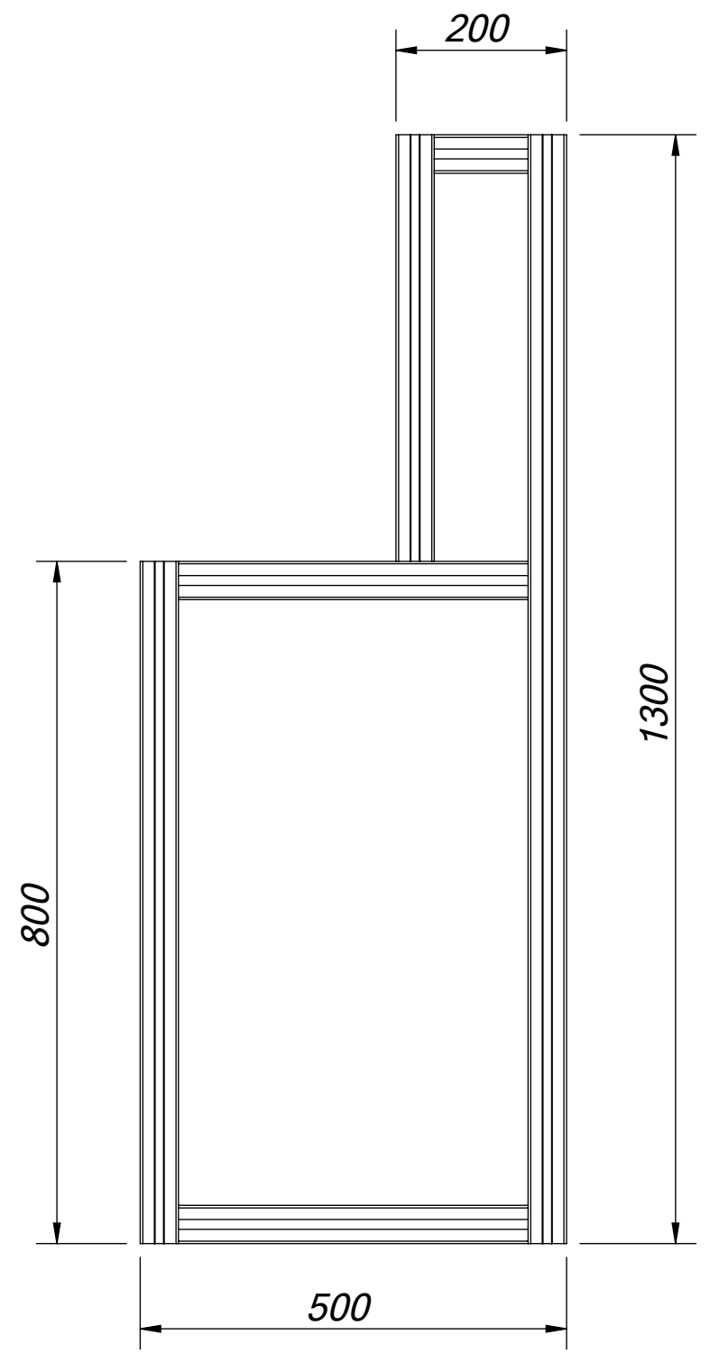
SIDE VIEW
