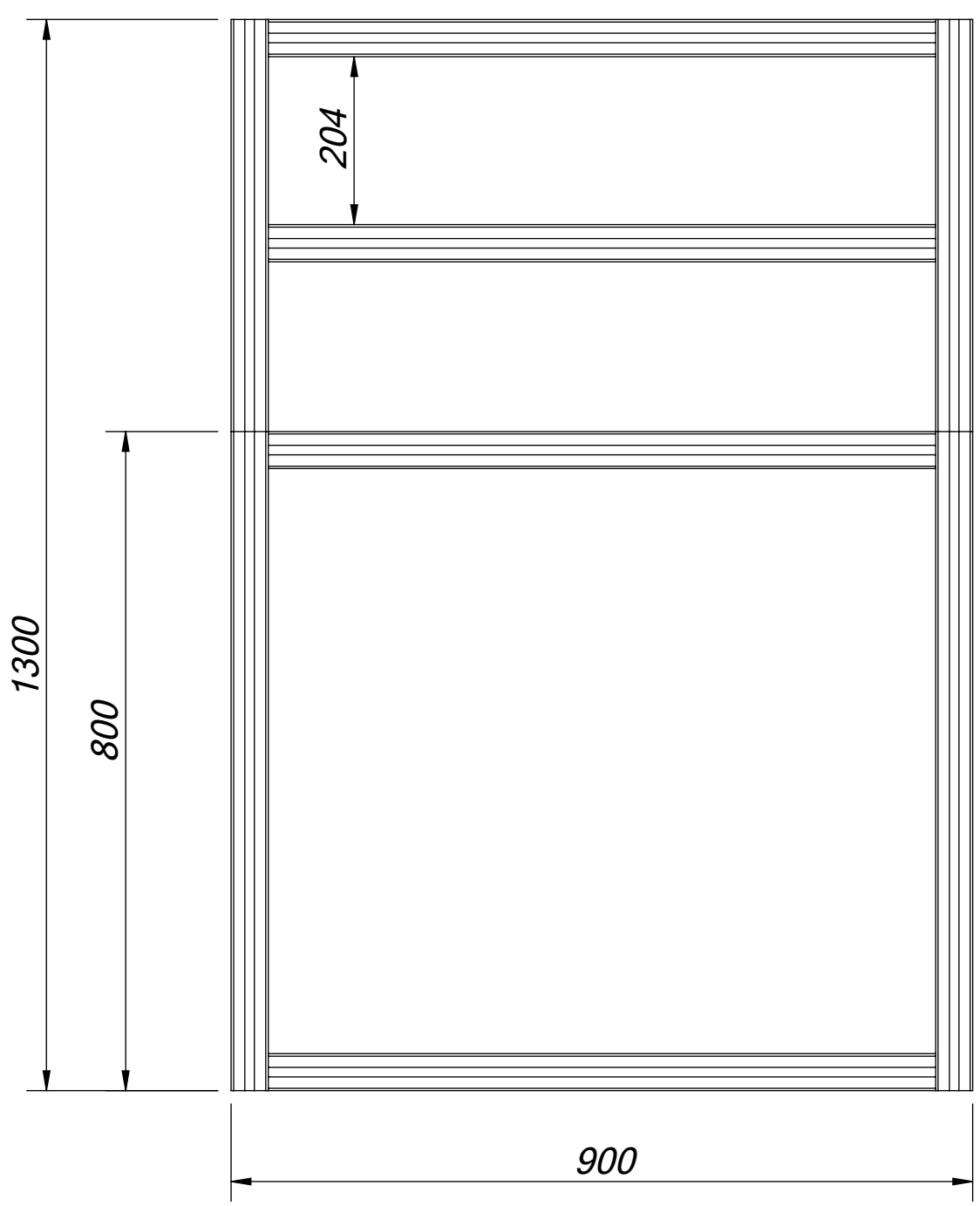
FRONT VIEW
