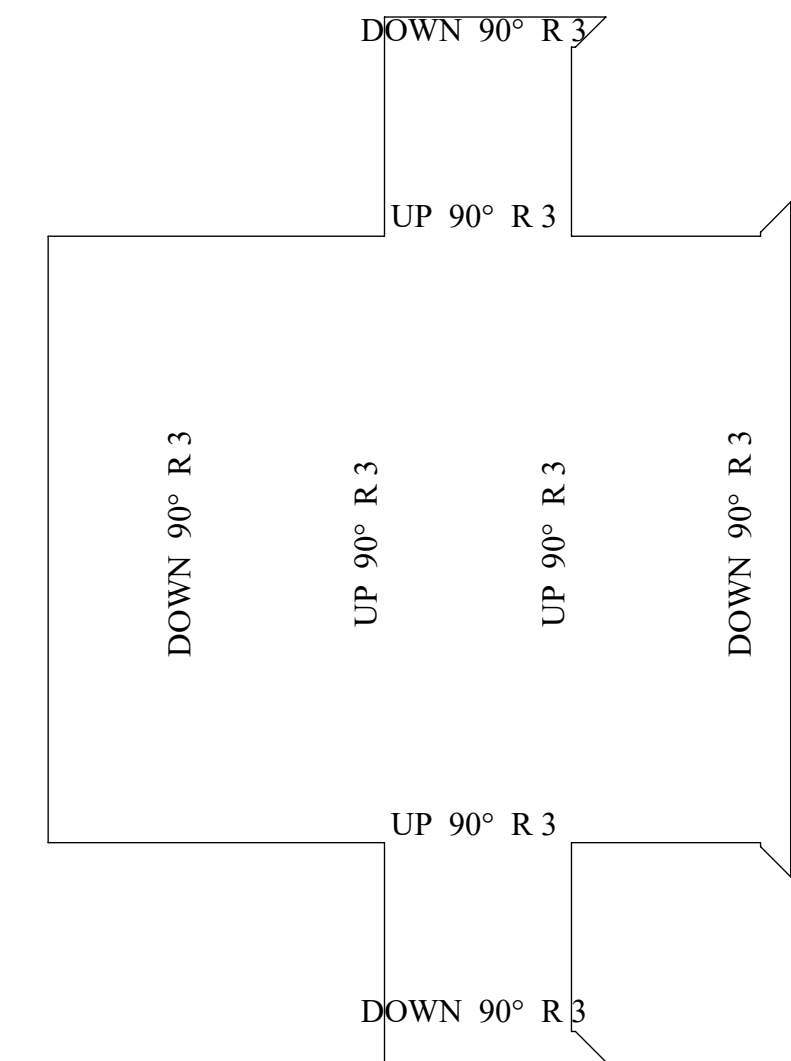
Flat pattern
