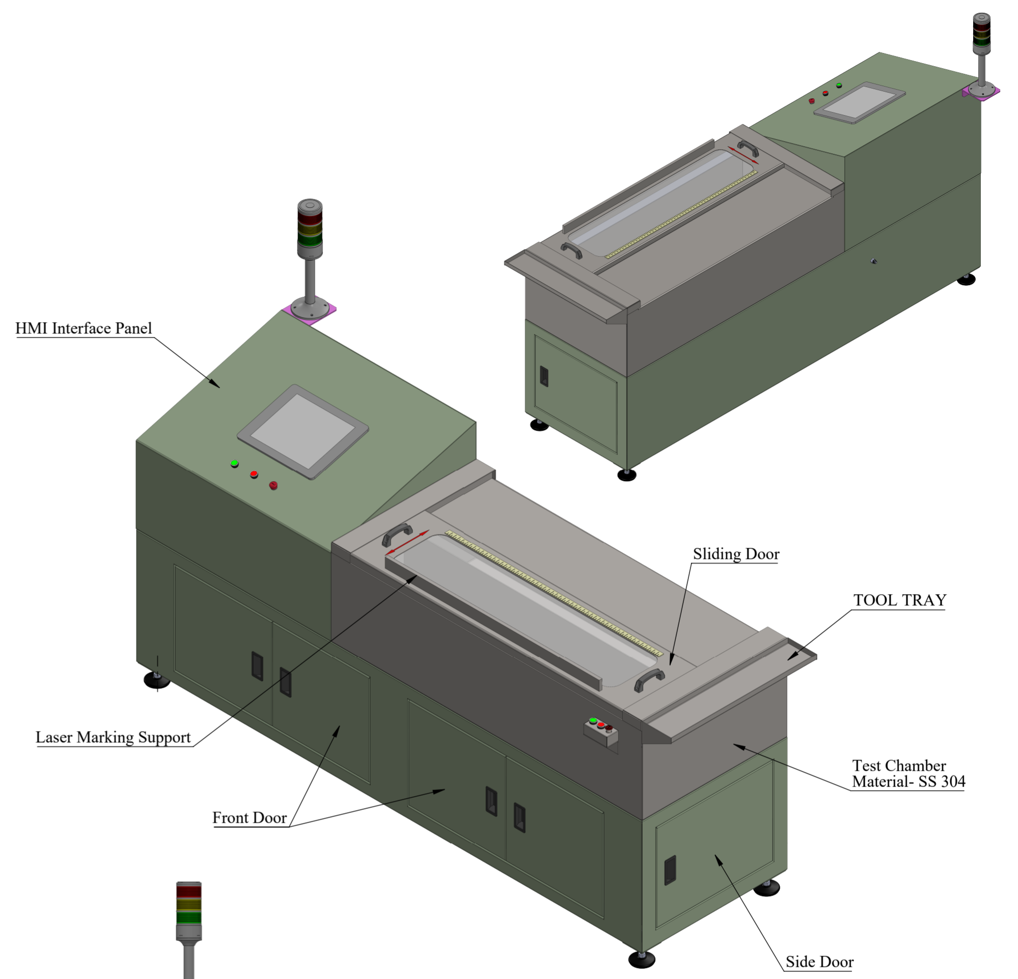
ISOMETRIC VIEW
