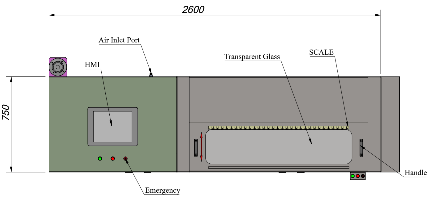
TOP VIEW
