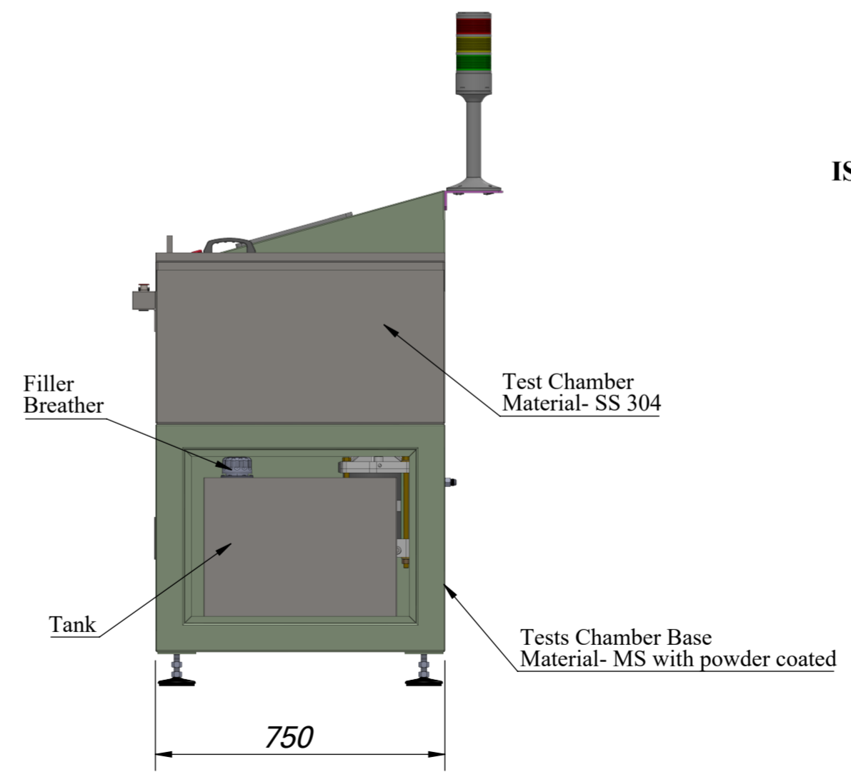
SIDE VIEW
