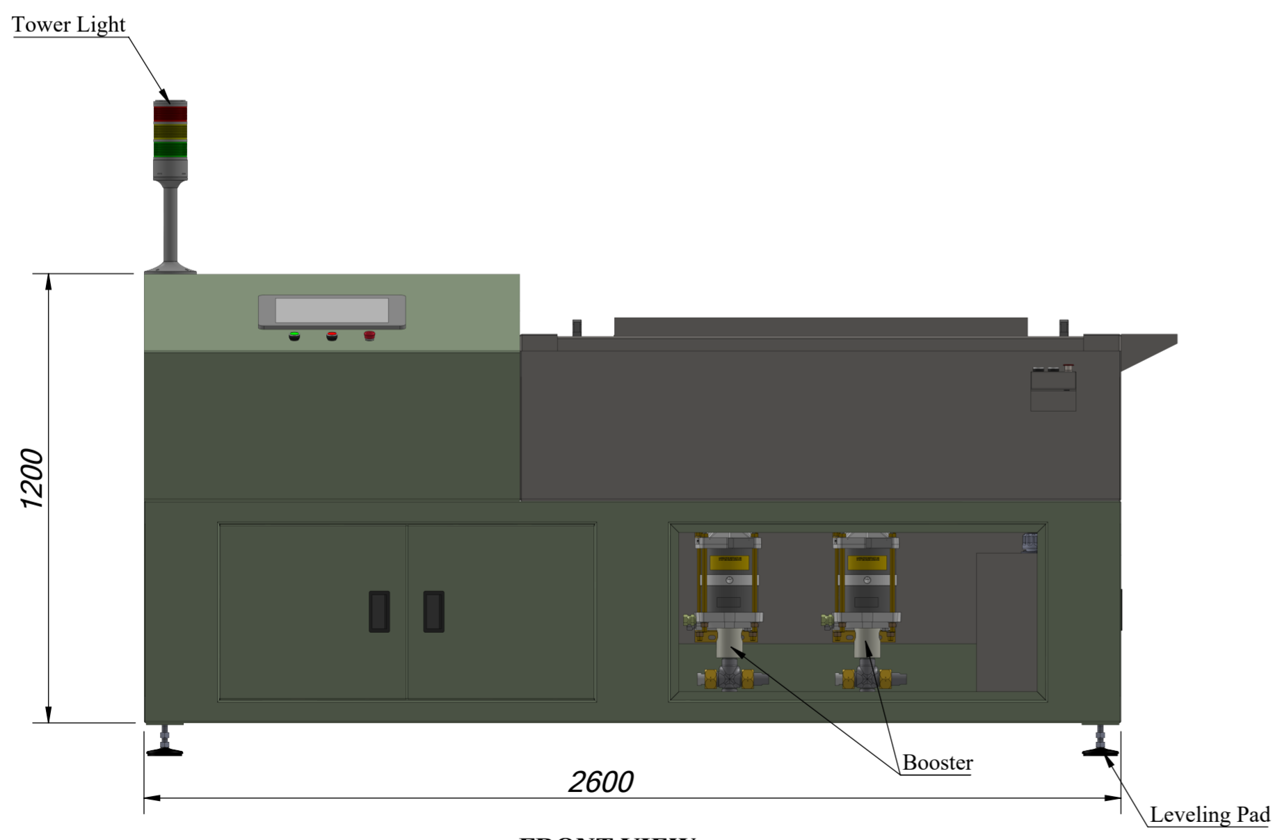
FRONT VIEW
